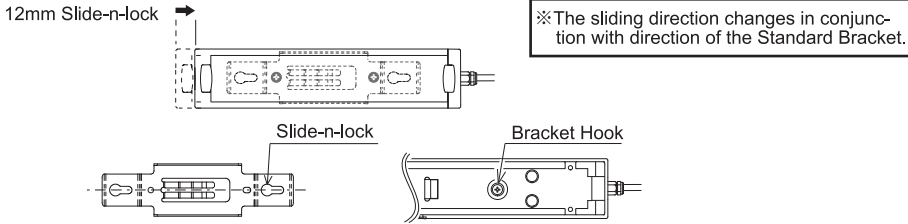
Figure 4. Slide Installation -1
