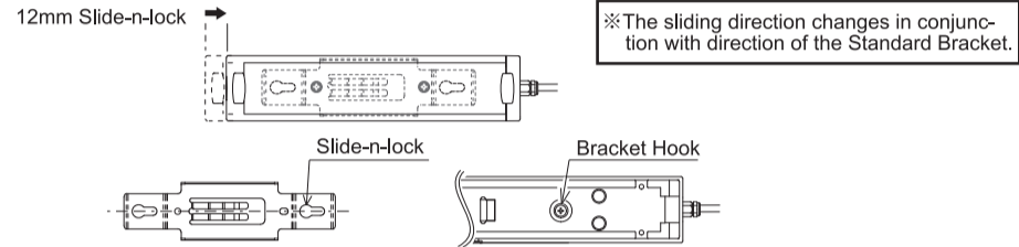
Figure 4. Slide Installation -1
