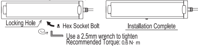
Figure 5. Installation -2
